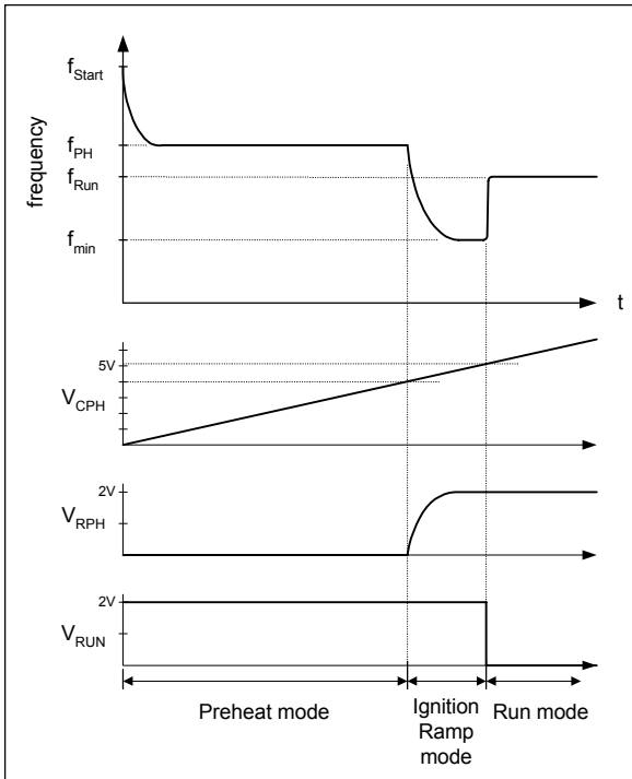
Figure 4: IR2167 Ballast Control Sequence
